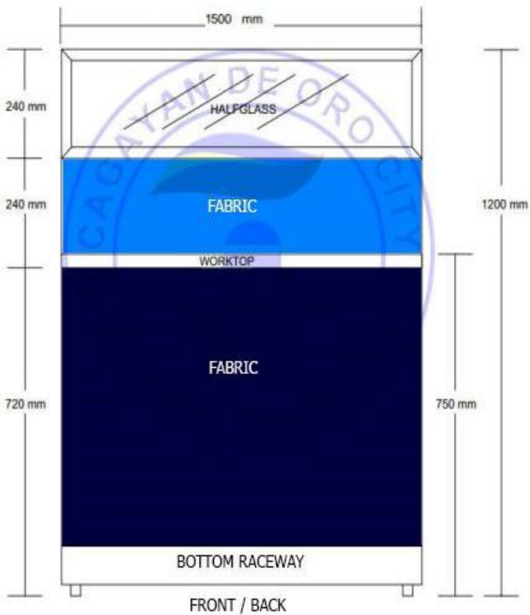
FIGURE 1.2 - 1 UNIT FABRIC PANEL WITH HALF GLASS AND BOTTOM RACE WAY (1200mm HIGH X 1500mm WIDTH )
