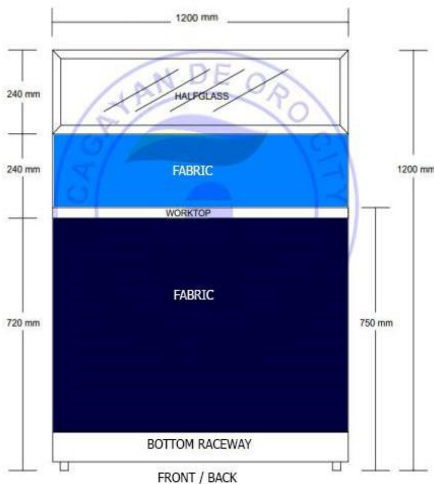
FIGURE 1.1 - 23 UNITS FABRIC PANEL WITH HALF GLASS AND BOTTOM RACE WAY (1200mm HIGH X 1200mm WIDTH )
