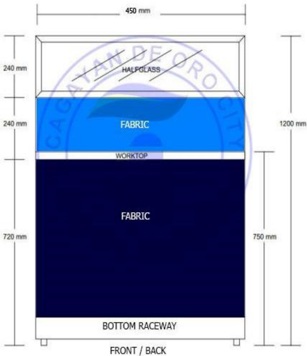
FIGURE 1.6 - 4 UNITS FABRIC PANEL WITH HALF GLASS AND BOTTOM RACE WAY (1200mm HIGH X 450mm WIDTH )
