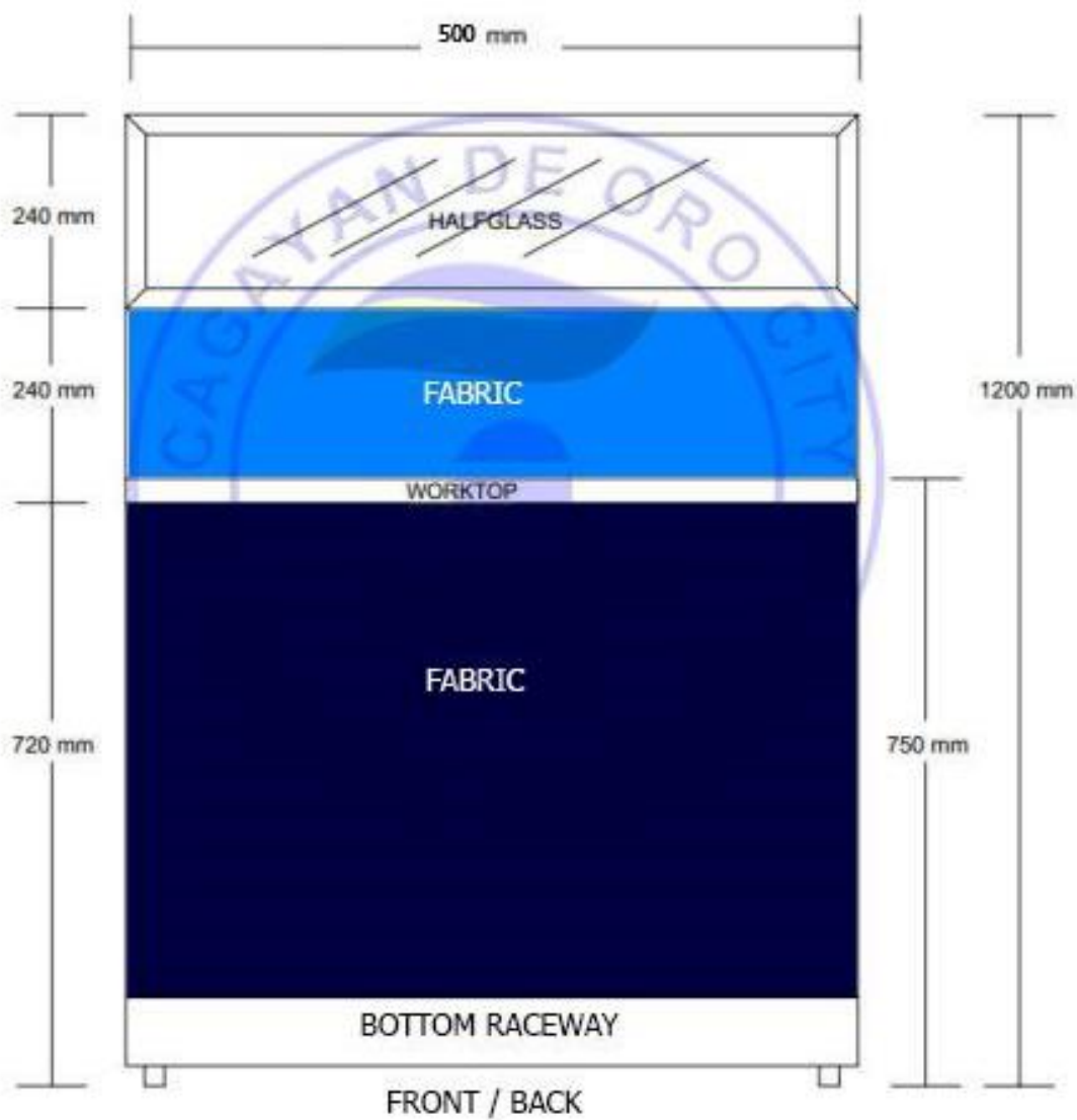
FIGURE 1.5 - 27 UNITS FABRIC PANEL WITH HALF GLASS AND BOTTOM RACE WAY (1200mm HIGH X 500mm WIDTH )
