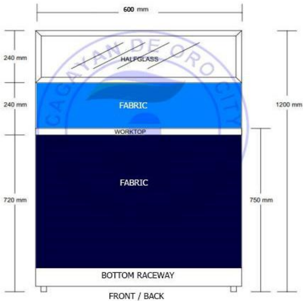
FIGURE 1.4 - 8 UNITS FABRIC PANEL WITH HALF GLASS AND BOTTOM RACE WAY (1200mm HIGH X 600mm WIDTH )
