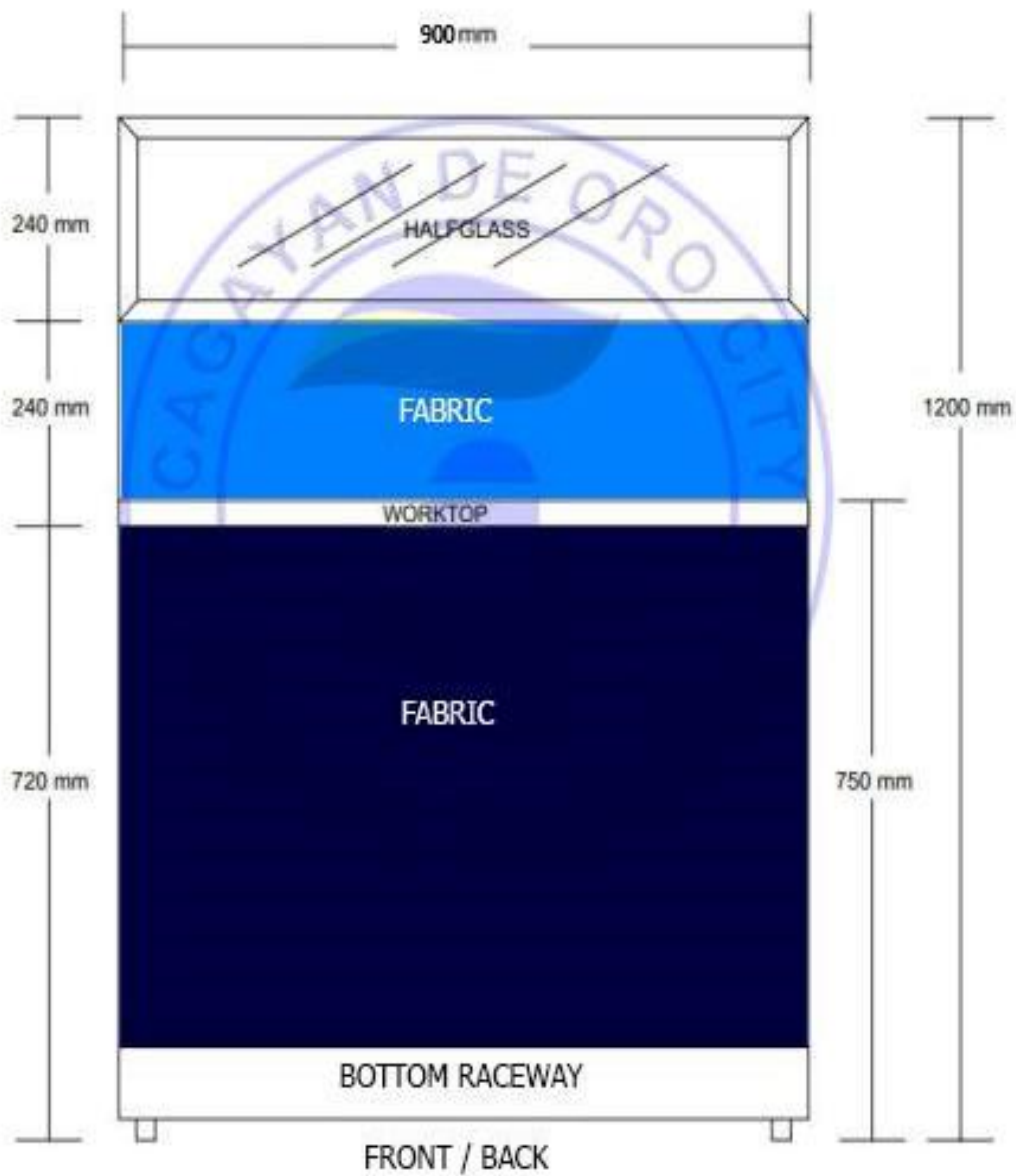
FIGURE 1.3 - 11 UNITS FABRIC PANEL WITH HALF GLASS AND BOTTOM RACE WAY (1200mm HIGH X 900mm WIDTH )
